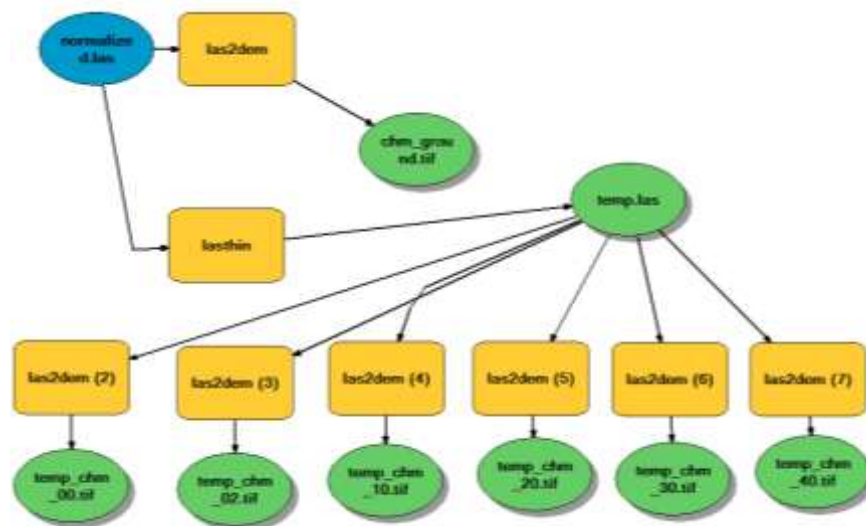
Fig. 3 – Model builder of the pit-free algorithm's work-flow
